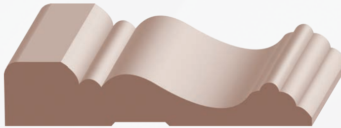
155BSP 11/16 x 3-1/4 Solid Pine Cape Cod Casing N
