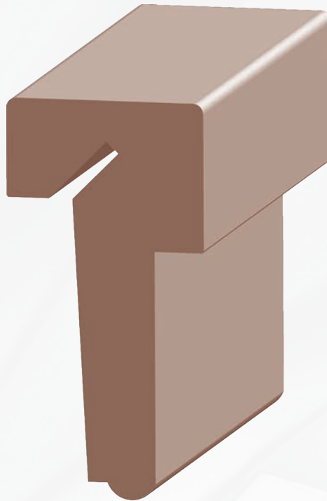
1-1/2 x 3-1/8 T-Astragal w/Weatherstrip Kerf
