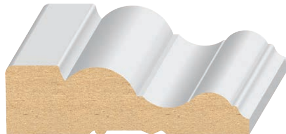
128MUL 11/16 x 2-1/2 Ultralight Mission/Bel-Air Casing N/S
