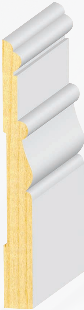
PR336FJ 9/16 x 5 Primed FJ Sierra/ Montecito Base N/S
