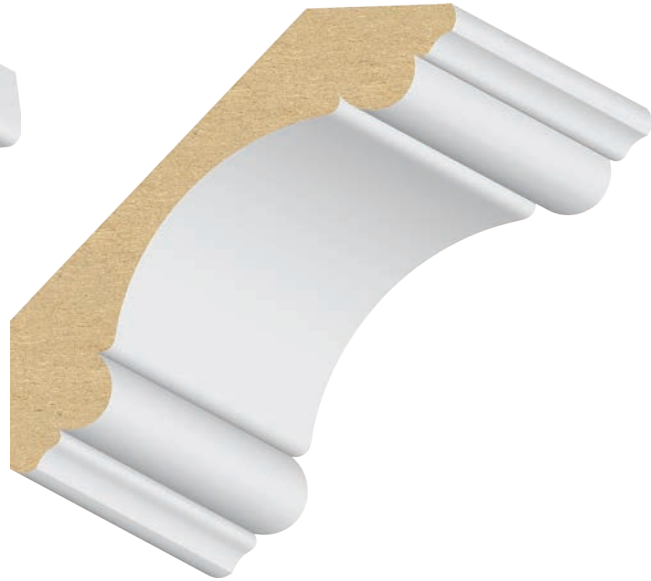
421MUL 3/4 x 3-3/8 Ultralight Double Bead Carolina Crown N/S
