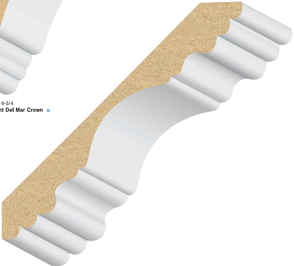
437MUL 13/16 x 6-7/8 Ultralight Santa Clara Crown N/S
