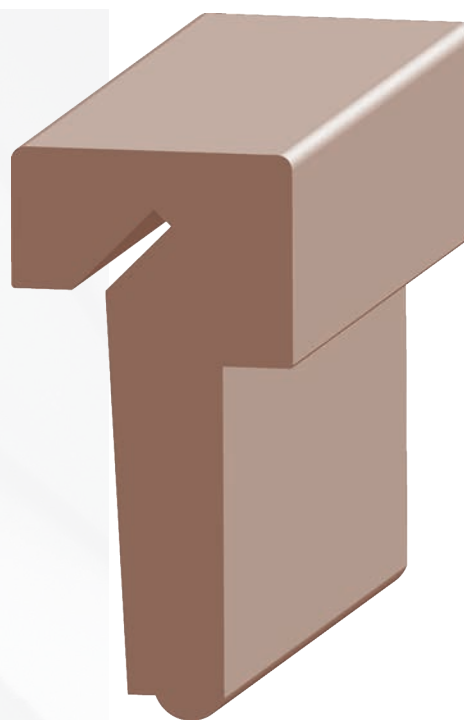
667VG 1-1/2 x 3-1/8 VG Fir Contemporary T-Astragal w/Weather Strip Kerf for 1-3/4" Door N/S (Q-Lon sold separately)
