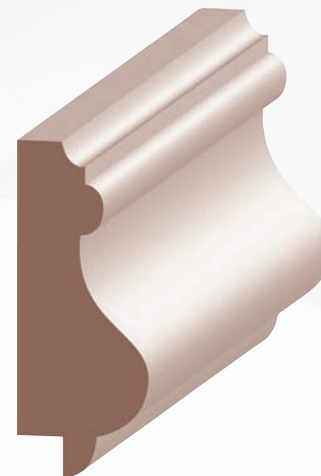
11/16 x 1-3/4 Panel Cap [with 1/4" Rab't]
