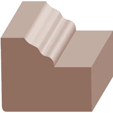
841R 1-1/4 x 1-1/2 Redwood Brick Mold N PR841R 1-1/4 x 1-1/2 Primed Redwood Brick Mold N
