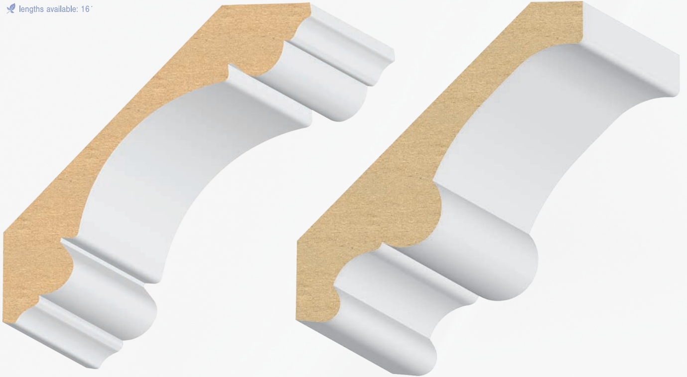
423MUL 7/8 x 4-5/8 Ultralight Double Bead Carolina Crown N/S 423BMUL 11/16 x 4-5/8 Ultralight Double Bead Carolina Crown N/S
