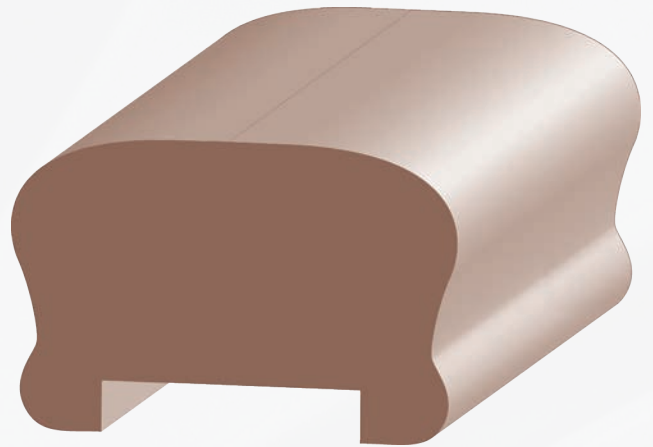
F925PL 1-1/2 x 2-3/8 Doug Fir Standard Handrail s with 1/4 x 1-1/4 Plow
